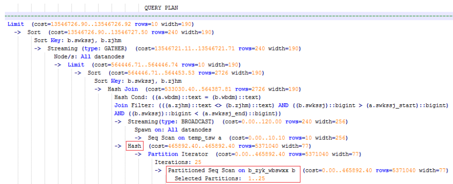
Figure 13-7 Using an unlogged table (2)
