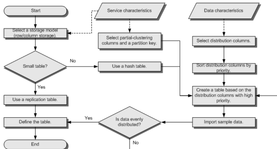
Figure 13-5 Defining a table
