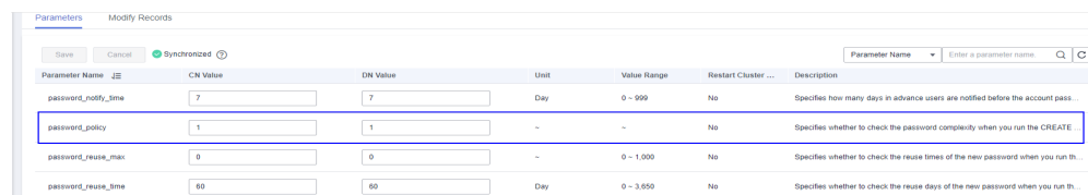
Figure 5-1 password_policy
