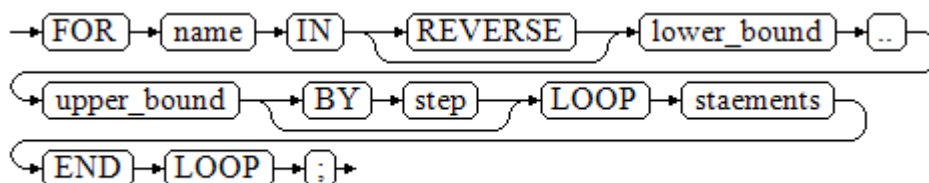
Figure 9-21 for_loop::=
