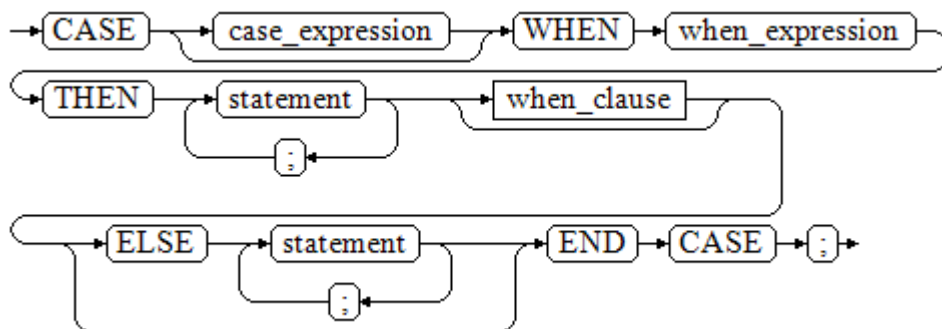
Figure 9-24 case_when::=
